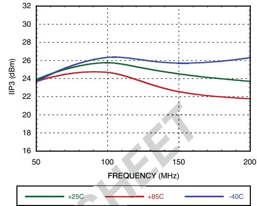
Figure 44. IIP3 vs. IF Frequency @ RF=900 MHz, VGATE=5V
