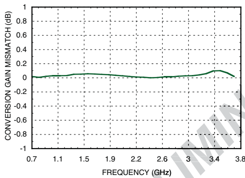
Figure 39. Low Side LO Conversion Gain Mismatch @ VGATE=5V [1]
