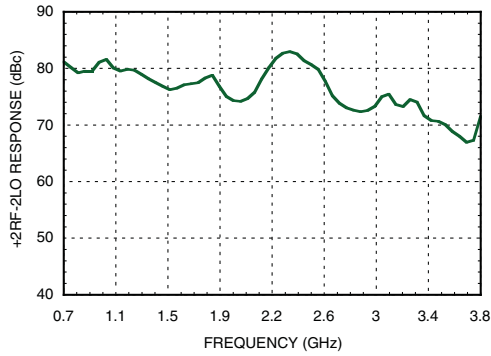
Figure 13. +2RF -2LO Response vs. Frequency over Temperature [1][2][3]
