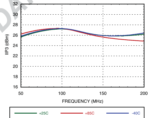
Figure 46. IIP3 vs. IF Frequency @ RF=1900 MHz, VGATE=5V
