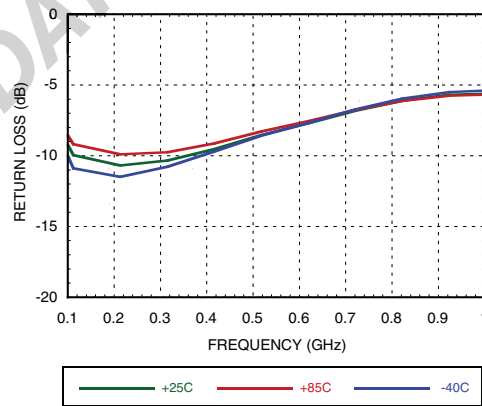
Figure 16. IF Output Return Loss vs. Frequency over Temperature [3][4]
