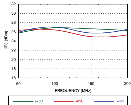
Figure 48. IIP3 vs. IF Frequency @ RF=2400 MHz, VGATE=5V
